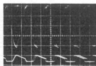
⑮ Top: FL2 output .1 \mu S/cm, .1V/cm Bottom: ICB-10 .1 \mu S/cm, 2V/cm
